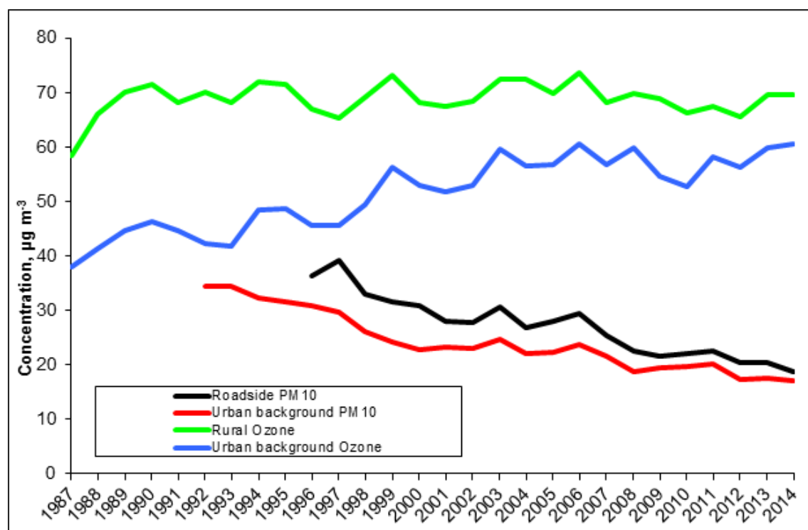
Figure 2 - Annual levels of PM 10 and Ozone in the UK, 1987 to 2014
